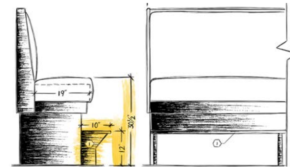
BAR HEIGHT W WOOD STEP
