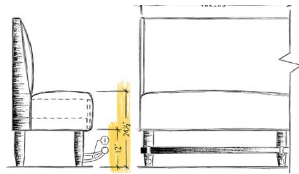
COUNTER HEIGHT W FOOT RAIL (BLACK, STAINLESS, BRASS)
