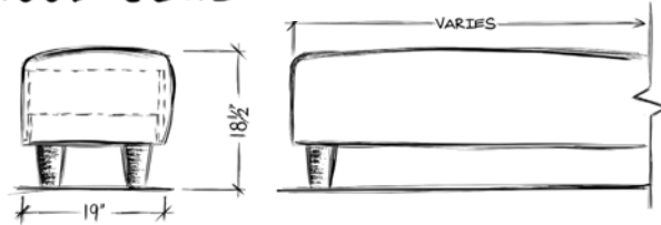
BIG SEAT, WOOD LEGS
